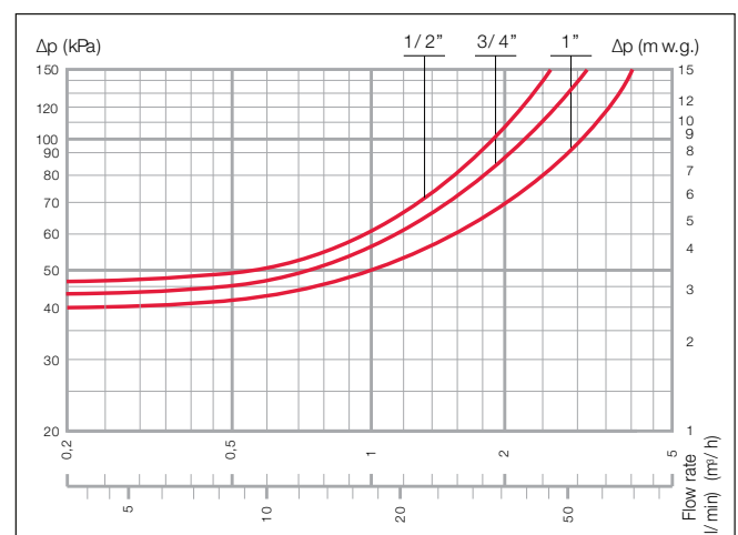
This chart shows curves at a 300kPa differential; curves for other settings are similar. The curve shifts slightly to the left for a smaller differential and to the right for a greater differential.
